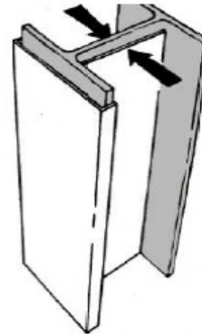
3) Push the web sections in to conform with the inside of the pile.
