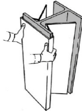
2) Square up the edges of the jacket scored to accommodate each end of the flange (full length of the jacket).
