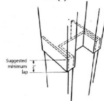
7) As each section is installed, lap as shown in Fig. no. 7 until desired length of pile is covered.
